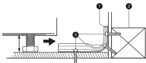
❶ Support antibasculement
