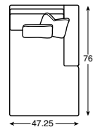
LTD5248-91-FB RAF Chaise Full Back W 47.25 D 76 H 33.5
