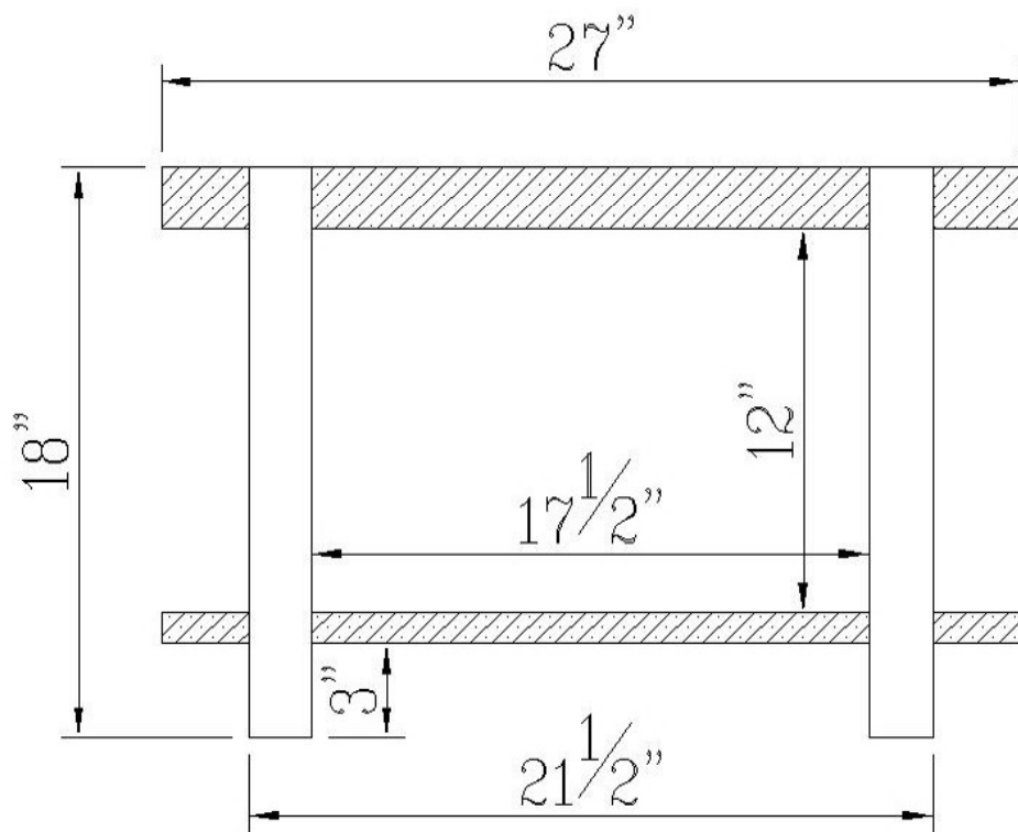
AMSA1320 Modesto – Cube Coffee Table
