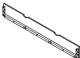
Front Panel
