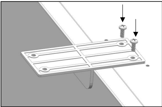
Fastener
