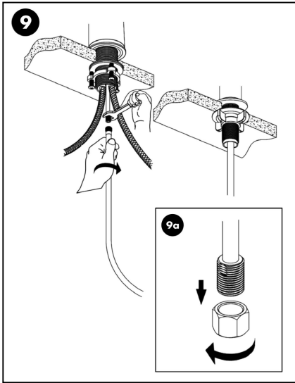
Tighten the hardware.
