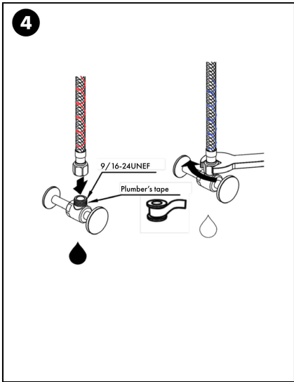
Secure the hoses to the hot (red) and cold (blue) lines appropriately.
