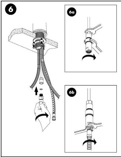
Secure the hardware into place.
