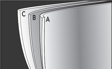
3-Layer Design: A. 18/10 Stainless Steel B. Aluminum C. Copper
