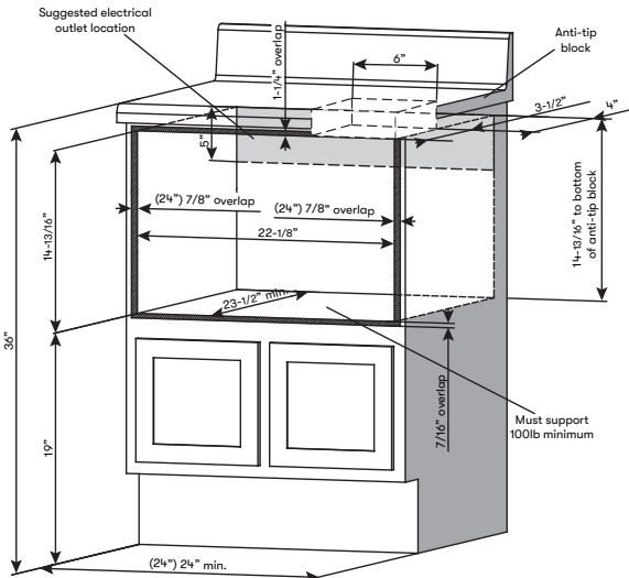
CABINET CUT-OUT
