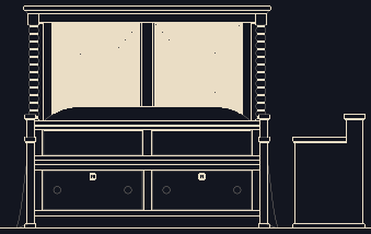
KING 667 HEADBOARD 82 1/8 x 4 3/8 x 60 068 ELDERS STORAGE BENCH 80 1/4 x 19 x 28 1/2
