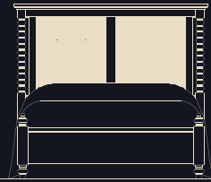
QUEEN 557 HEADBOARD 65 1/8 x 4 3/8 x 58 3/4 755 LOW PROFILE POSTER FOOTBOARD 62 5/8 x 3 5/8 x 22
