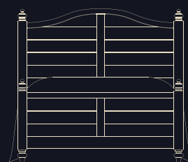
QUEEN 559 HEADBOARD 62 5/8 x 3 5/8 x 58 955 HIGH POSTER FOOTBOARD 62 5/8 x 3 5/8 x 31 1/4
