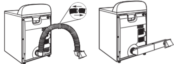
Over-The-Top installation (also available with one offset elbow). Semi rigid venting used in this example. Periscope installation
