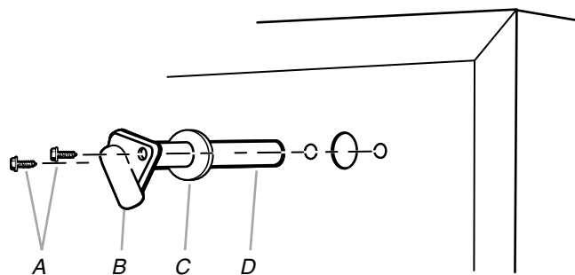
A. Hex head sheet metal screws B. Spout
