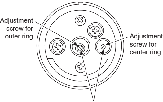
Adjustment screws for multi-ring burner only
