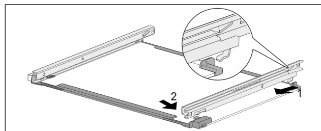
Fig. 116 Glass shelf with rails
