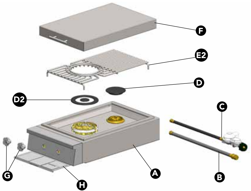
FIGURE 13 Double Cooktop with Power Wok Burner
