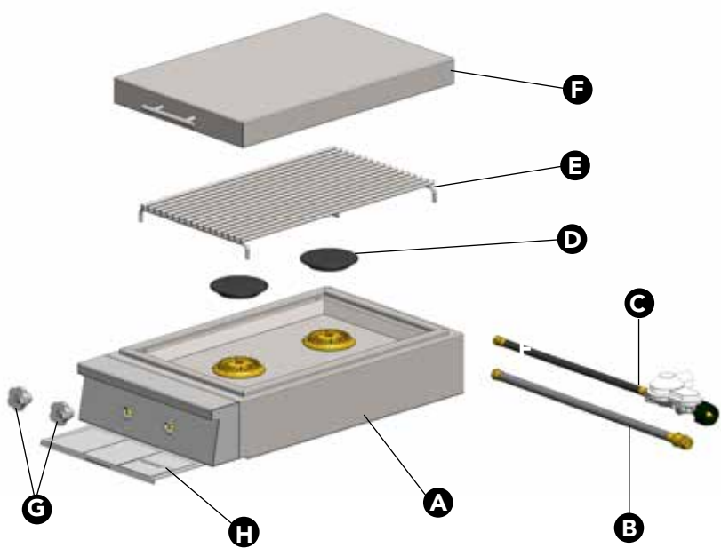
FIGURE 12 Double-Burner Cooktop
