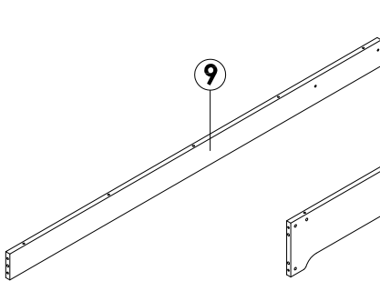
BOTTOM TOP RAIL (FRONT) ( 1 PC / SET ) CARTON 3 OF 4
