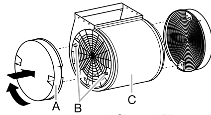
A. Charcoal Filter B. Pins C. Blower Motor
