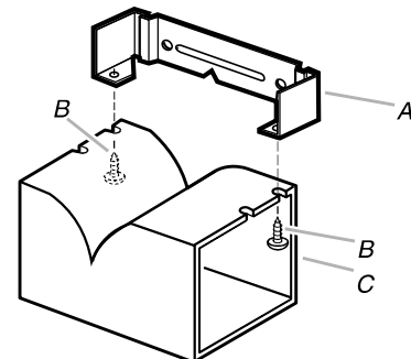
A. Vent cover bracket B. Assembly screws C. Deflector
