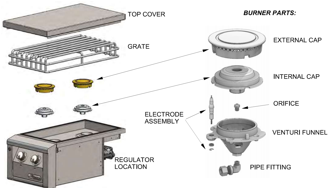
Figure # 1 SIDE BURNER BODY
