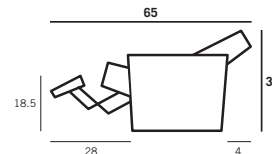
Side View (wall saver mechanism, fully reclined)
