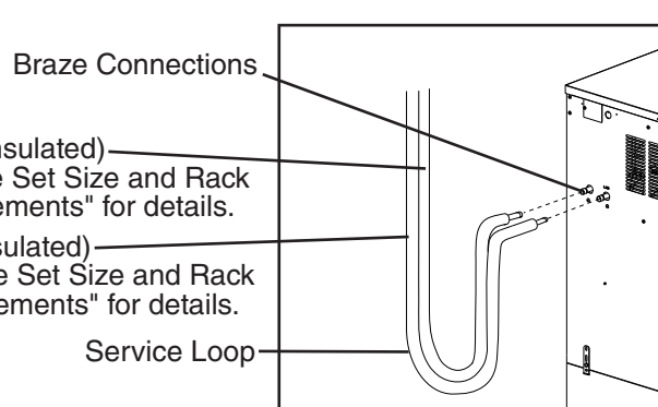
Icemaker Braze Connection
