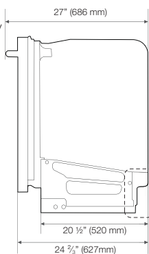
Side view (DMT800 series/ DMT610 series/ DMT400 series)
