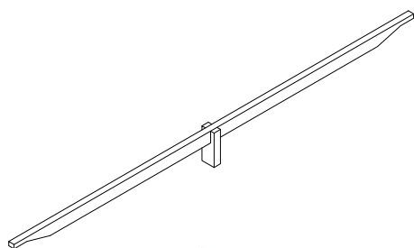
P4. Center Support (x2)
