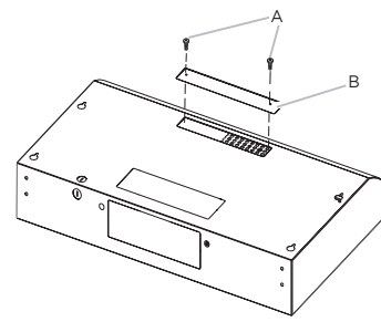
A. Screws (2) B. Recirculation cover plate
