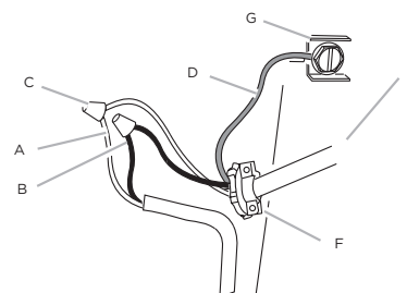
A. White wires B. Black wires C. UL listed wire connector D. Green (or bare) ground wire E. Home power supply cable or power cord accessory kit F. UL listed or CSA approved \frac{1}{2} " strain relief G. Green ground screw
