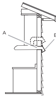
Wall Venting
