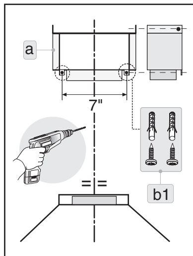
Fig.3: Center the air diverter A in the middle of the hood and position it as high as needed. Follow the indicated quotas to drill the holes and fasten the diverter using the screws and expansion plugs b1 .
