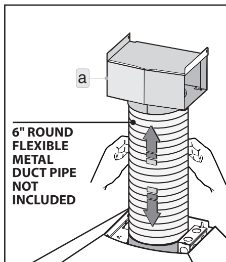
Fig.4: Once the air diverter has been inserted into the bracket and fastened to the wall connect the flexible ( 6" ROUND FLEXIBLE METAL DUCT PIPE NOT INCLUDED ) pipe to the diverter, use duct tape to seal.
