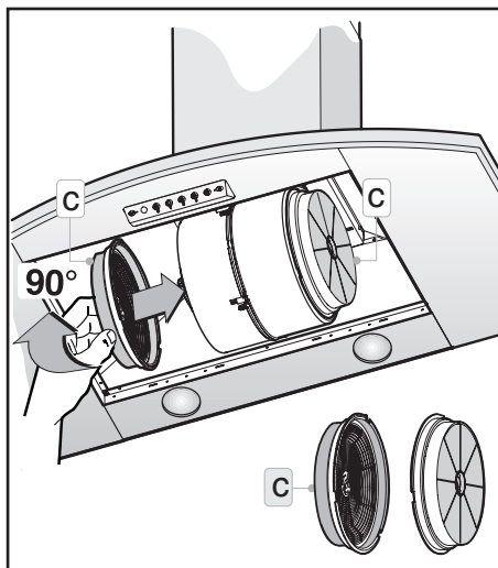
Fig.7: The filters C must be applied to the suction unit inside the hood, centering them inside of it and turning them 90° until they snap into place.
