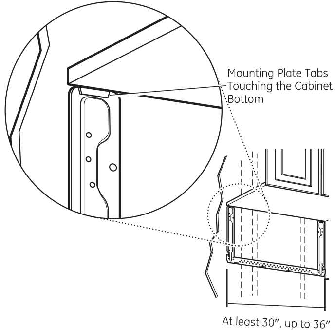
Plate position – beneath flat bottom cabinet
