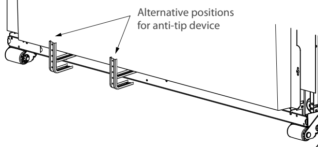
Fig. 12.25 Anti-Tip bracket
