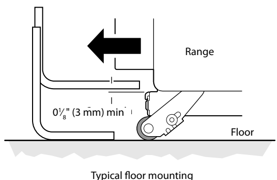
Fig. 12.25 Anti-Tip bracket
