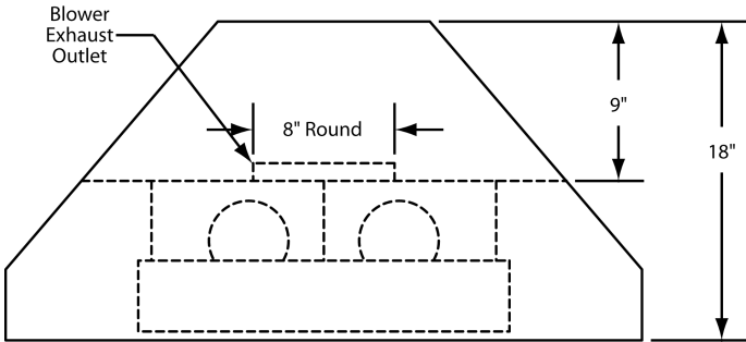
600 CFM B200 Dual Blower (Top View)
