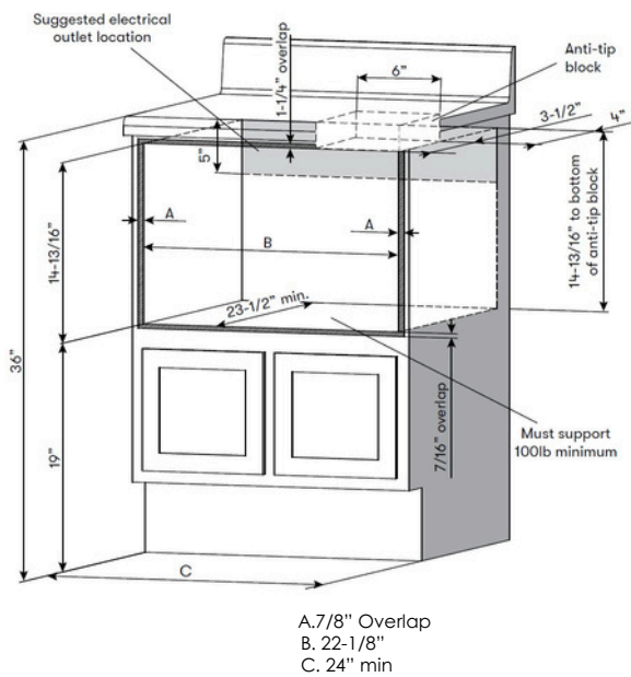
CABINET CUT-OUT FOR STANDARD INSTALLATION
