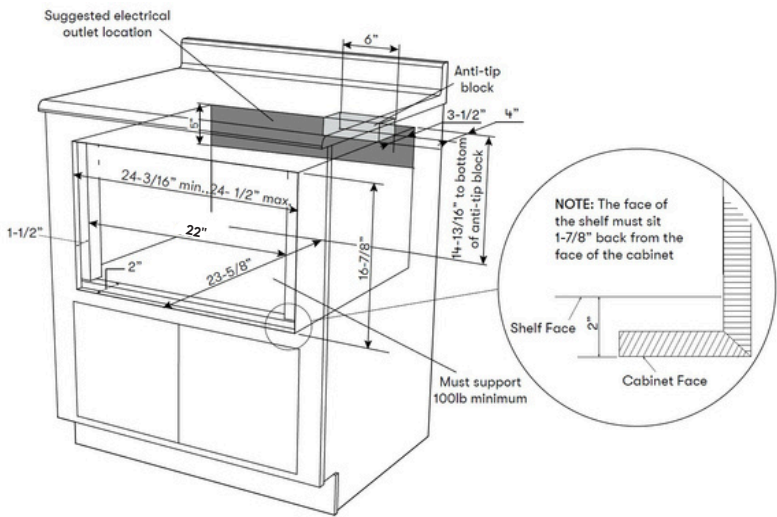
CABINET CUT-OUT FOR FLUSH MOUNT INSTALLATION
