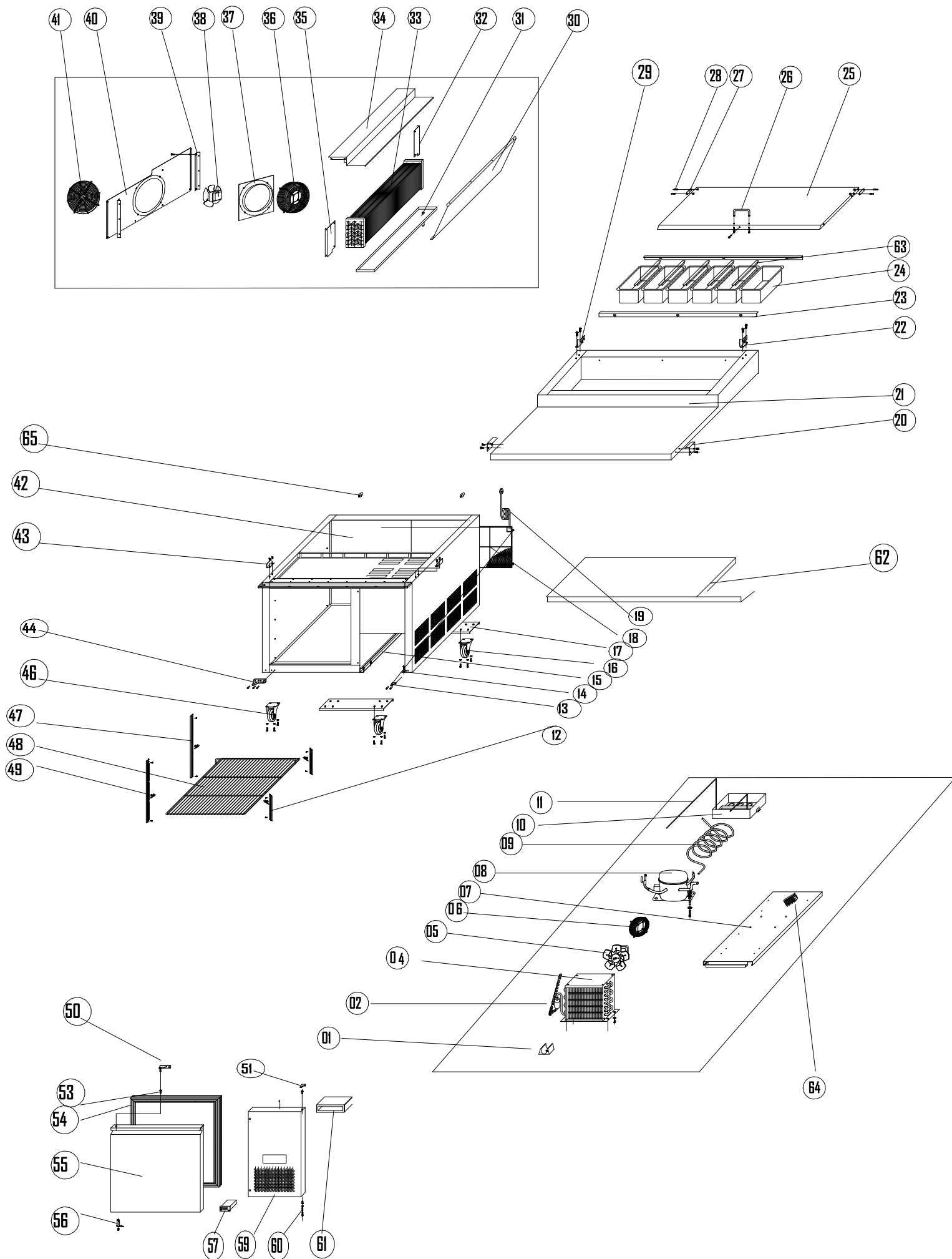
EXPLODE OF KCHPT50.6
