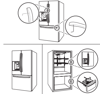
Disassembling/Assembling
