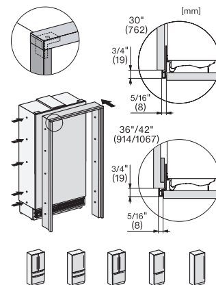
KFMC3632R+L, KFMC3642R+L, KFMC3836R+L, KFMC3834R+L, KFMC3858FD, MasterCool III, integration, neutral, installation
