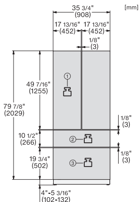
KFMC3846FD, MasterCool III, front view (US)
