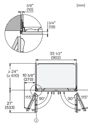
KFMC3846FD, MasterCool III, PACS, with stainless steel front, top view (US)
