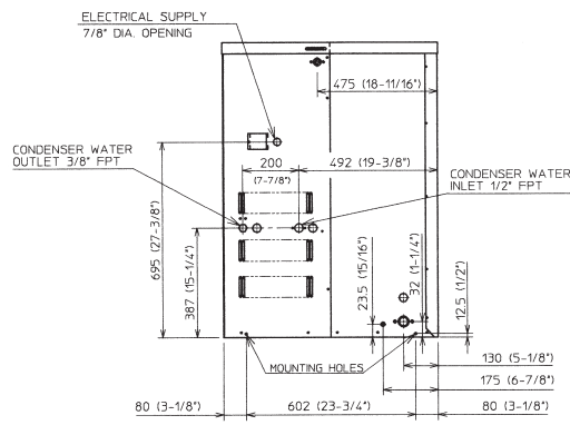
WATER-COOLED
