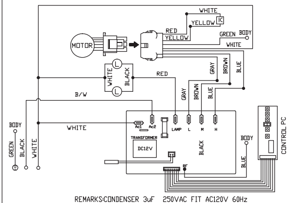
CIRCUIT DIAGRAM(SINGLE)
