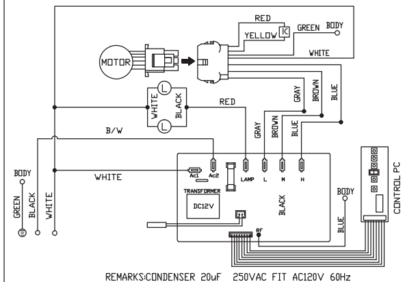
CIRCUIT DIAGRAM(SINGLE)
