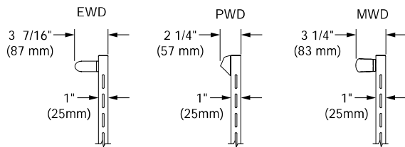
Handle Dimensions
