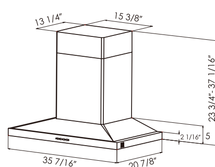
▲ EMS9018 Product Dimensions
