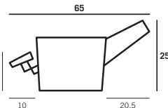
Side View (standard mechanism, fully reclined)
